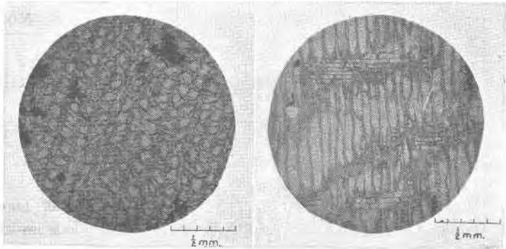
Figure 1. Photomicrograph of transverse section of calcified log from Pittsburgh Coal.
