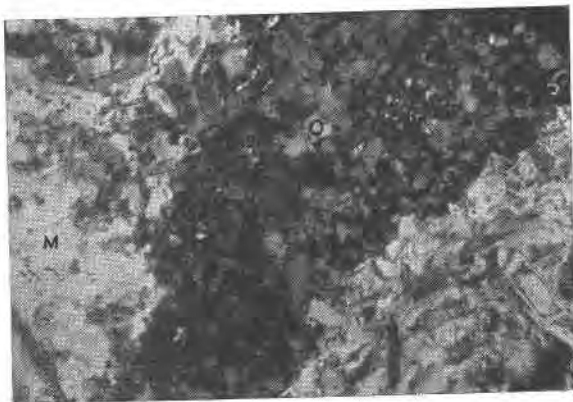
PLATE I A. Veinlet of orthoclase (O) cutting muscovite (M). The small laths on the muscovite are of sericite. Microphotograph with crossed nicols. \times 100 .
