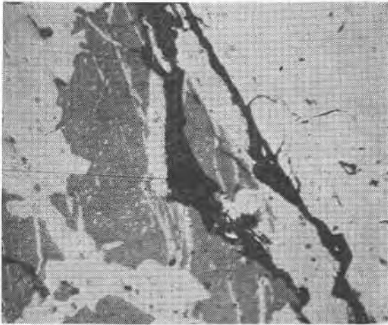
FIG. 2. Older sphalerite (gray), containing chalcopyrite blebs (white), partly replaced by chalcopyrite. Black spots are holes. Nicsols not crossed. Magnification 400 diameters.
