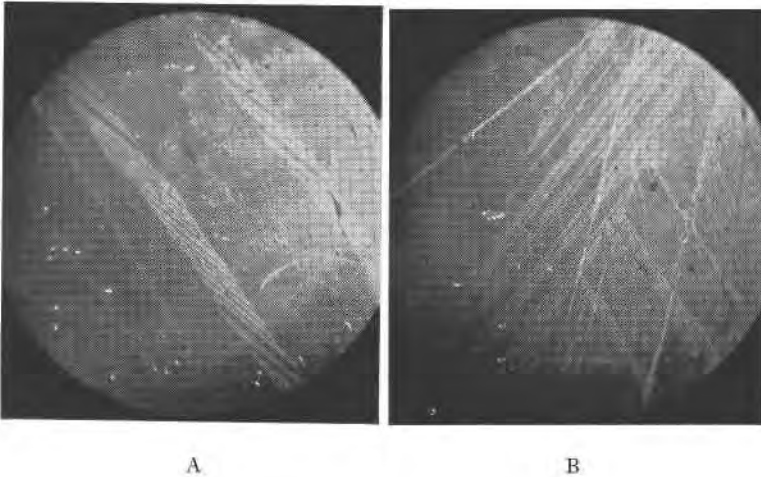
FIG. 3. Echelon twin lamellae, on surface of chalcopyrite polished parallel to c axis, and brought out by etching 3 minutes with etchant. Crossed nicols, \times 28 . Figure 3A shows a set of two wide and one narrow group of echelon twins , with a cubanite band almost parallel to these. The faint, dark, broad bands running across the field, transverse to the echelon twins are the grid twins as seen on this surface. Figure 3B shows two different group directions in the echelon twins , and also shows the interchangeability of individual direction within an echelon group. This photograph also illustrates the intersection of cubanite bands and echelon twins .
