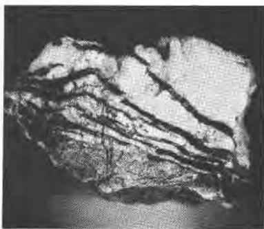
FIG. 10. Another view of quartz vein material, showing gashes of later piedmontite. This is purer than other types found in the Tucson Mountains and was chosen for the chemical analysis. Note portion of wall rock at bottom. \times 0.7 .
