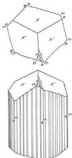
FIG. 3. Lower end of a Klein-Spitzkopje crystal of type 1, showing the form \frac{3}{2} and the striated appearance.
