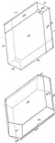
FIG. 2. Plan and orthographic projection (26° rotation, 25° tilt). A common habit of ammonium molybdo-ditellurate.
