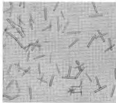
FIG. 12. Crystals of calcium sulfate hemihydrate ( \text{CaSO}_4 \cdot \frac{1}{2}\text{H}_2\text{O} ). Compare with the more common crystals of microchemical gypsum in Fig. 11. \times 220 .
