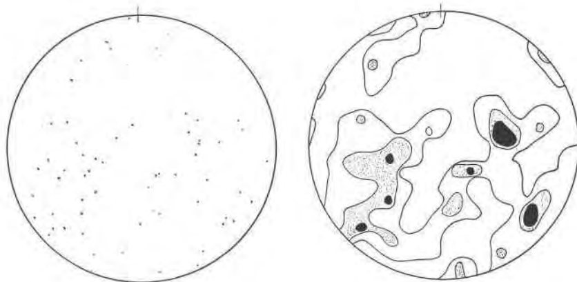
FIG. 13. Quartzose slate. Petrofabric diagram of a quartzzone phase in some slates near Deadwood, S. D., with 57 quartz axes. The contour intervals are 0, 1.8, 3.5, 5.3%. Statistical analysis: general test P = .35 ; zone test P' = .82 (-),* .65 (80), .77 (170). The general test and the zone test in all three positions all indicate random distribution of orientation. The results of the zone test show that the distribution is very uniform in every respect. In view of the statistical data, it is doubtful whether a greater number of grains measured would discover any significant orientation. Specimen 14849, slide 7610, U.S. Geol. Survey collection.
