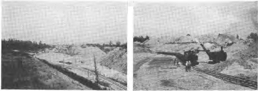
FIG. 1 (left). A general view of the clay workings at Attapulugus, Georgia, showing the large amount of terrane mined in removing fullers earth. The spoil piles of old workings appear in the picture.
