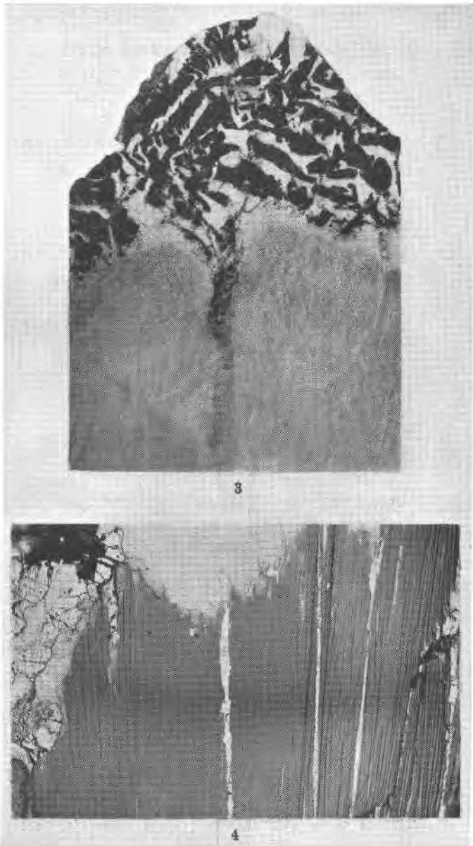
FIG. 3. Polished specimen illustrating the relations of albite-sphalerite to microcline. The lower half of the figure represents microcline cut by a vein of quartz. The narrow light-colored zone between microcline and sphalerite represents granular albite that has partly replaced microcline. Near the center sphalerite has replaced part of the quartz vein. 1/4 natural size.
