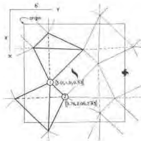
FIG. 4A. Nieuwenkamp's illustration of the structure of low cristobalite projected on (00\bar{1}) .
