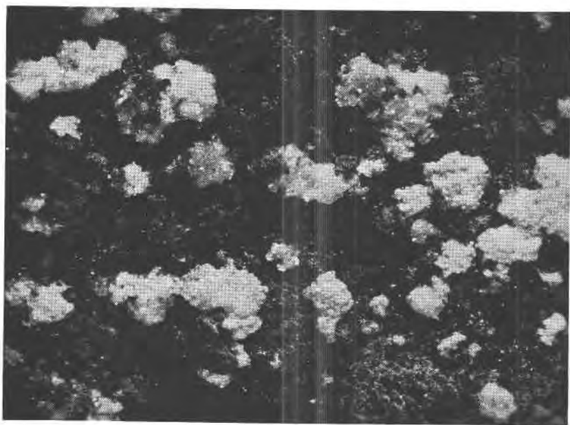
FIG. 1. Schroekingeringite on uraninite from Jáchymov. \times 8 .
