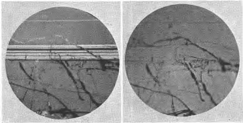
FIG. 1. The plagioclase crystal of example 1 showing the twin lamellae in contrasting illumination.
