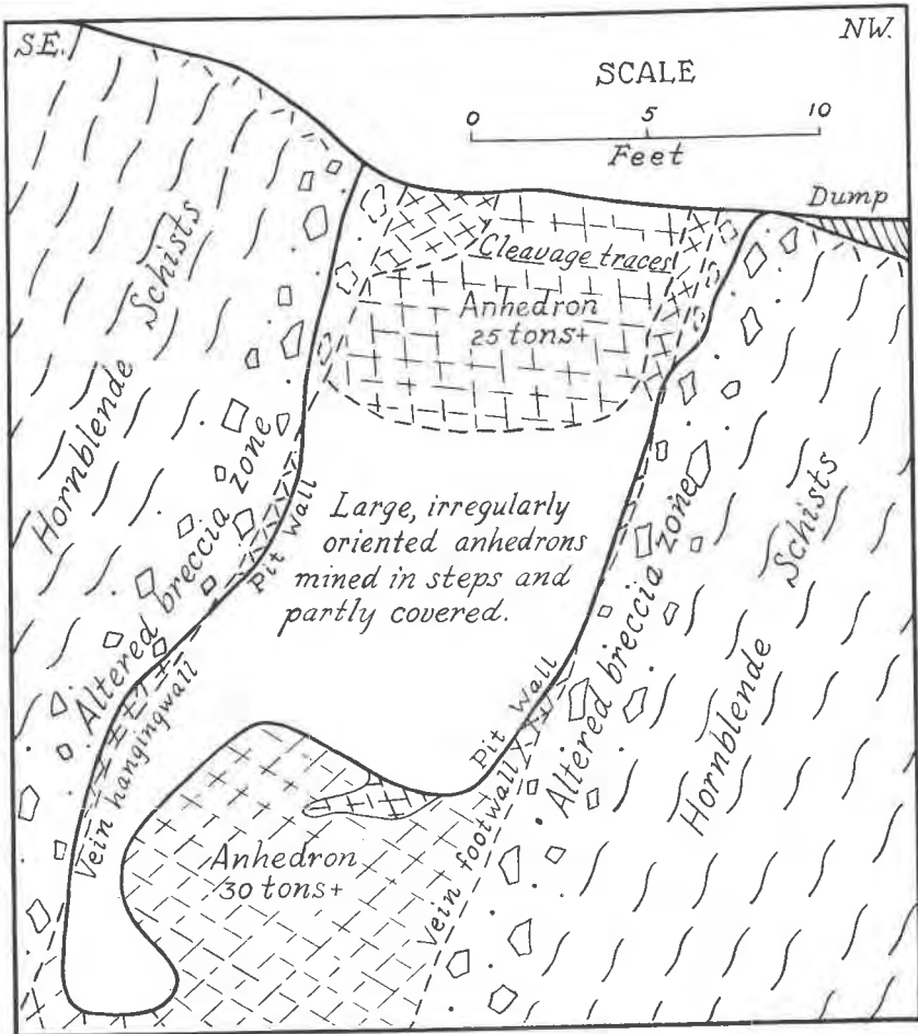
FIG. 2. Cross section of Iceland spar vein showing orientation and position of large anhedron crystals.
