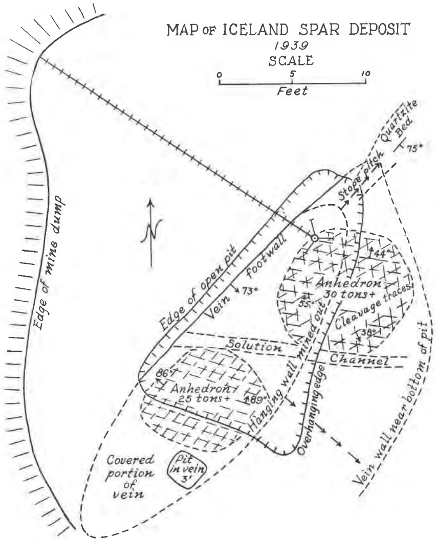
FIG. 1. Map of Iceland spar deposit.
