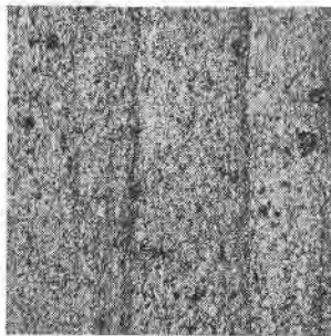
FIG. 4. Thin section of pyrite in coarse sulphur. Transmitted, ordinary, light. Magnification 4.2X.
