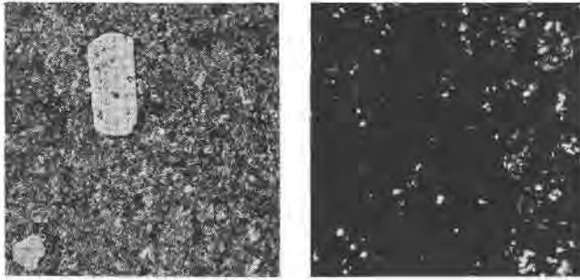
FIG. 2 (left). Phenocryst and groundmass replaced by pyrite in reflected light. Magnification 12.5X.
