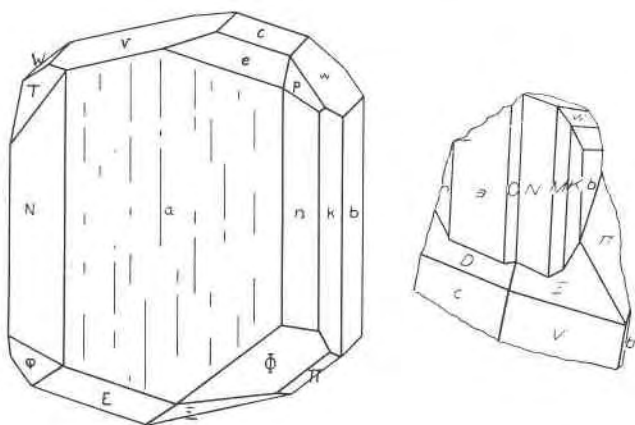
FIG. 1. Bellingerite—Chuquicamata
