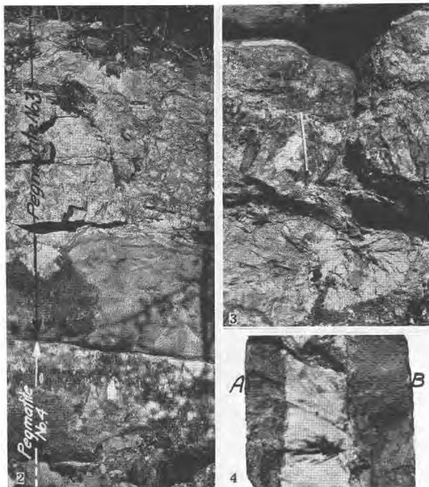
FIG. 2. A portion of the face of pegmatites Nos. 3 and 4. Note the fine-grained contact zone at the base of pegmatite No. 3 and the narrow radial band of muscovite near the top of pegmatite No. 4.
