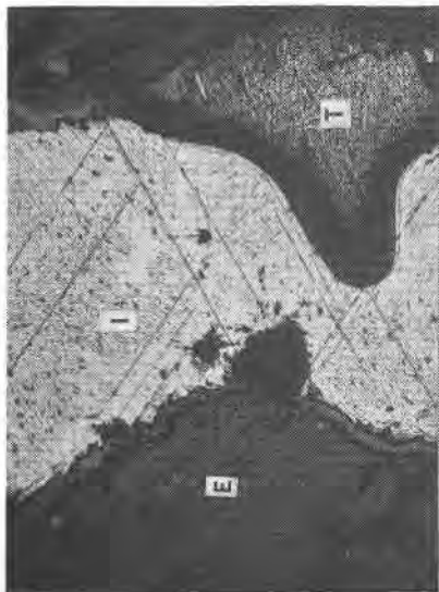
FIG. 3. Nickel-iron (I) etched with nitol, showing Neumann lines and pearlitic structure. Troilite (T) and enstatite (E). The border around the nickel-iron and the troilite is due to oxidation ( \times 100 ). Shallowwater meteorite.
