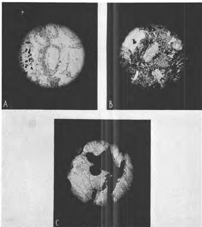
FIG. 5. Photomicrographs of three stages in alteration of a quartz monzonite inclusion in basalt.
