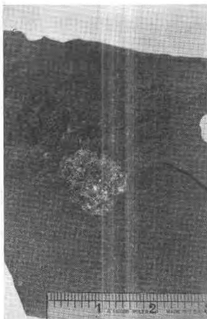
FIG. 2. Iron stained quartz-rich inclusion in basalt of the Bartolas group. Enclosure composed of a few grains of andesine with corroded margins, and many grains of strained quartz.
