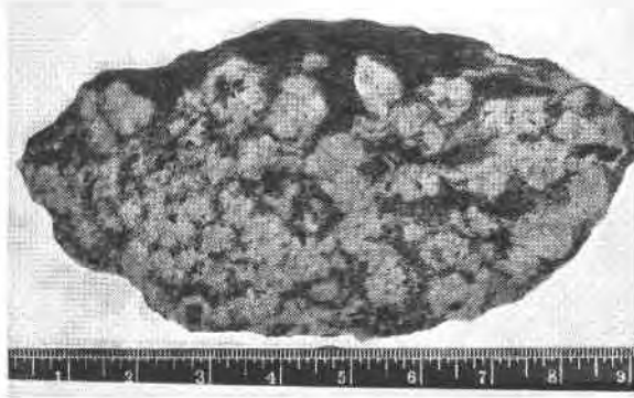
FIG. 5. Feldspar porphyroblasts and incipient orbicules in schist.
