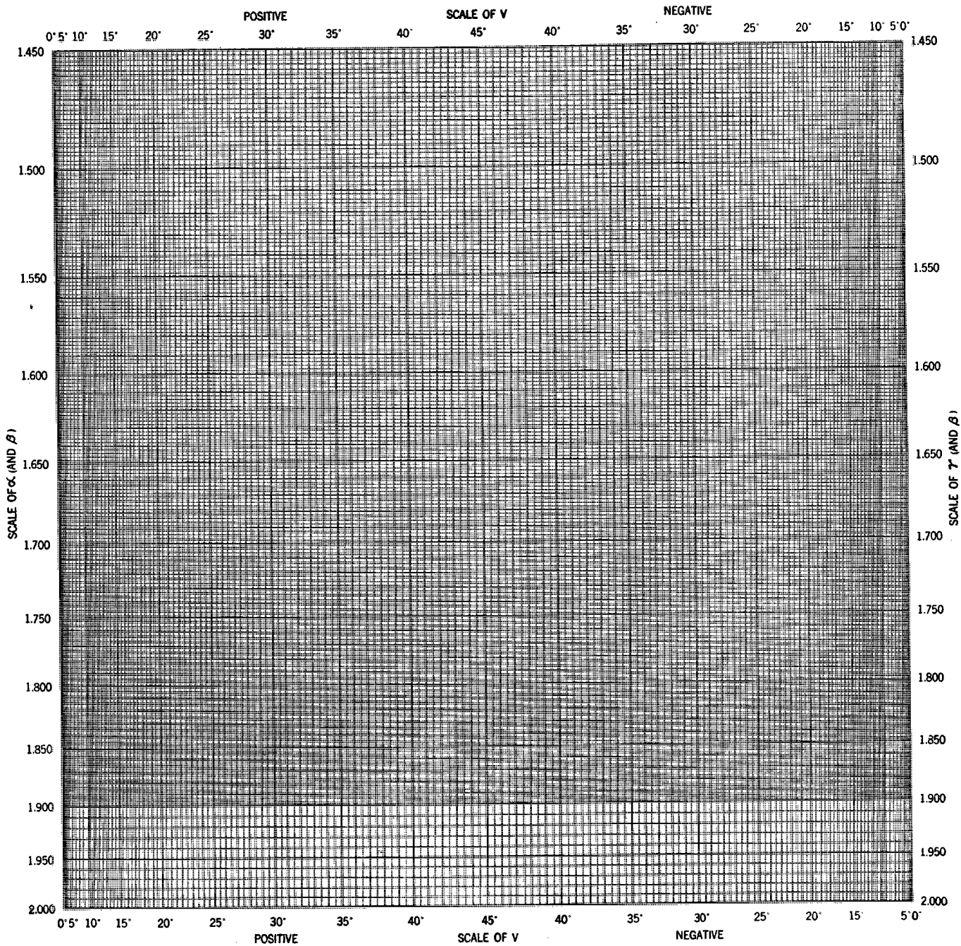
PLATE I. NOMOGRAM OF \sin^2 V_1 = \frac{\frac{1}{\alpha^2} - \frac{1}{\beta^2}}{\frac{1}{\alpha^2} - \frac{1}{\gamma^2}} AND \sin^2 V_2 = \frac{\frac{1}{\beta^2} - \frac{1}{\gamma^2}}{\frac{1}{\alpha^2} - \frac{1}{\gamma^2}}
