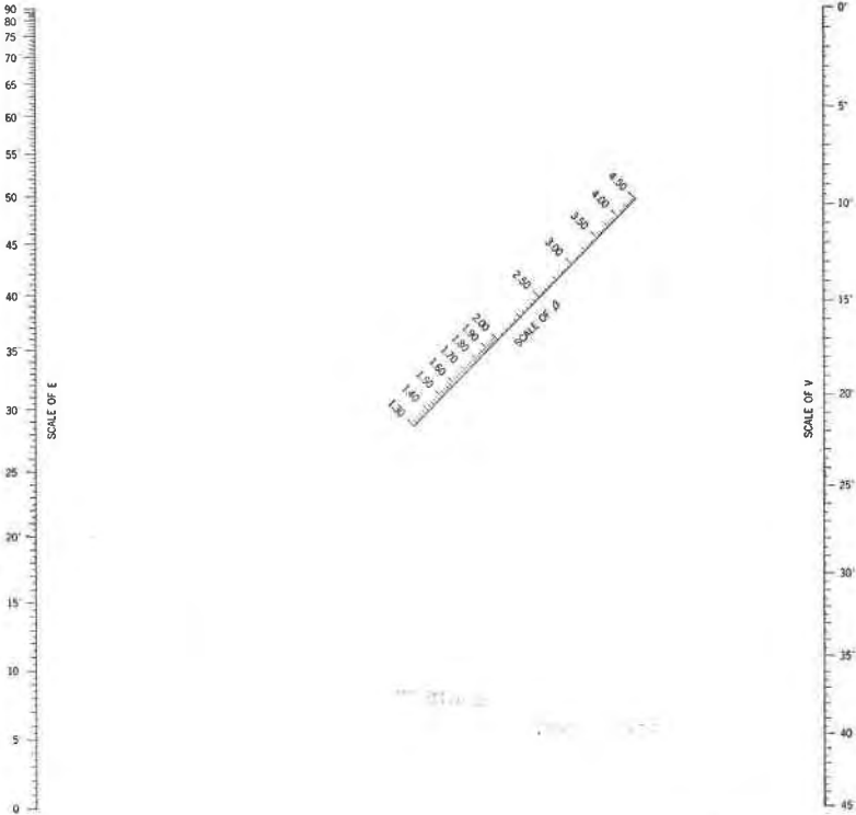
PLATE III. NOMOGRAM OF \sin E = \beta \sin V JOHN B. MERTIE, JR. U. S. GEOLOGICAL SURVEY
