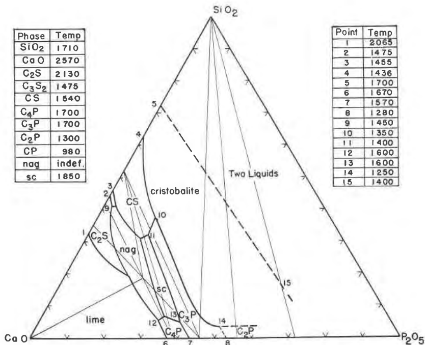
FIG. 3. Equilibrium diagram for the system \text{CaO-SiO}_2\text{-P}_2\text{O}_5 . Temperatures are approximate.
