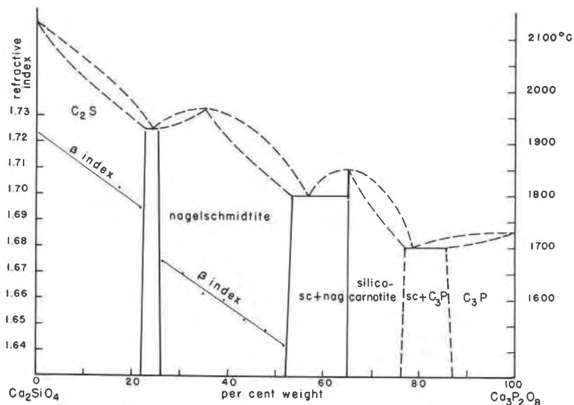
FIG. 4. Diagram showing probable equilibrium relationships in the system Ca_2SiO_4 - Ca_3P_2O_8 . Liquidus temperatures not definitely known. Extent of solid solution and variation in refractive index shown for calcium orthosilicate and nagelschmidite.
