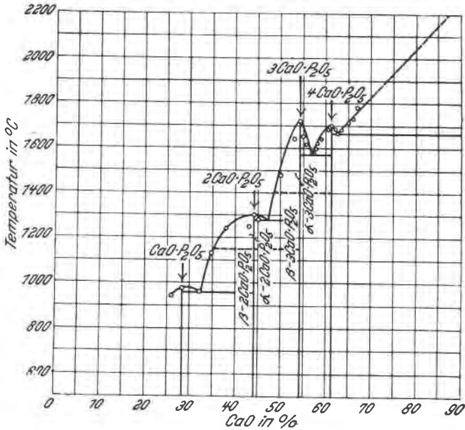
FIG. 1. System \text{CaO}-\text{P}_2\text{O}_5 from Körber and Trömel, Arch. Eisenhüttenwesen 1, 7 (1933).
