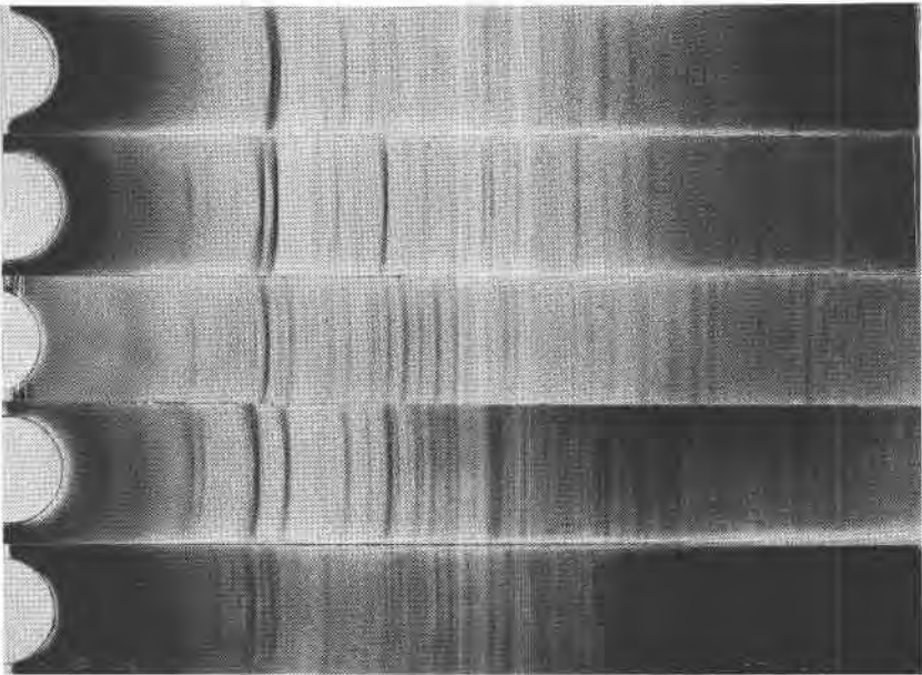
FIG. 6. X-ray powder diffraction patterns made with Cu radiation. Reading from top to bottom the phases are: \beta -calcium orthosilicate, nagelschmidite, silicocarnotite, \alpha -tricalcium phosphate, and tetracalcium phosphate.
