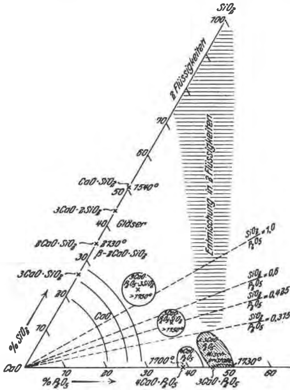
FIG. 2. Sketch for system \text{CaO-P}_2\text{O}_5\text{-SiO}_2 from Körber and Trömel, Arch. Eisenhüttenwesen , 1, 7 (1933).
