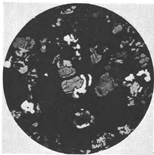
FIG. 5. Photomicrograph of thin section of remelted open hearth slag from Ensley Alabama. Magnification about 75 times. Crossed nicols. Gray grains are nagelschmidite white grains are silicocarnotite. Background is dark colored interstitial phase.
