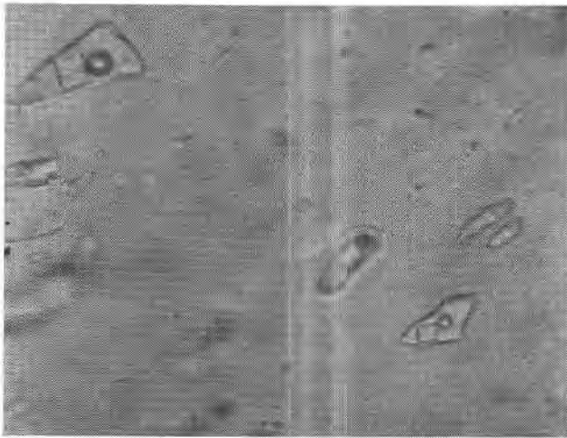
FIG. 9 (X400). Liquid-gas-halite inclusions in natural Colombian emerald.
