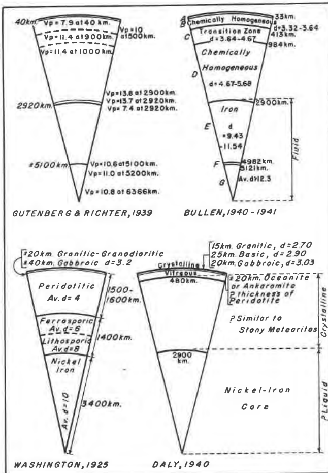
FIG. 2. Upper figures show geophysical data as interpreted by different authorities; lower figures show equivalent lithology as proposed by different men. d =density, Vp =velocity of compressional earthquake wave.
