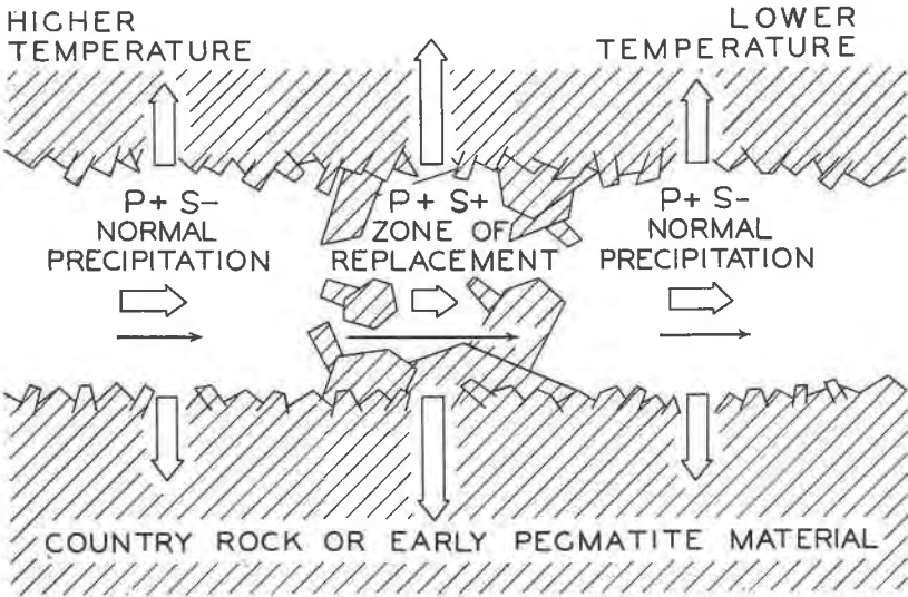
FIG. 1. Diagram to illustrate relations of precipitation, solution and replacement with the temperature gradients along a pegmatite thorofare.
