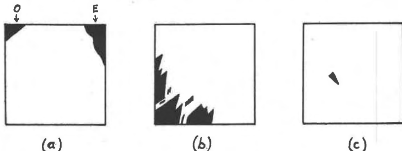
FIG. 1. Oscillator-plates with areas optically and electrically twinned. 1(a) Optical (O) and electrical (E) twinning. 1(b) and (c) Optical twinning.
