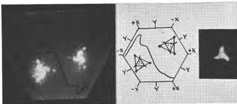
FIG. 17. Light figures on electrically twinned Z-sections showing three typical equilateral triangles formed by three sets of spots useful for orientation purposes. The outer set of brightest spots form equilateral triangle with sides parallel to Y-axes. The fainter spots with tails form a triangle with sides parallel to X-axes. The propeller-like figure becomes more distinct with long etching and shows hand of crystal (both right-handed in this case).
