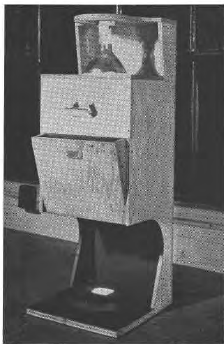
FIG. 21. Twinoscope. Consists simply of a spot-light on turntable and viewing slot approximately 22^\circ from the normal for determining useful portions of electrically twinned wafers by differences in light reflectance.
