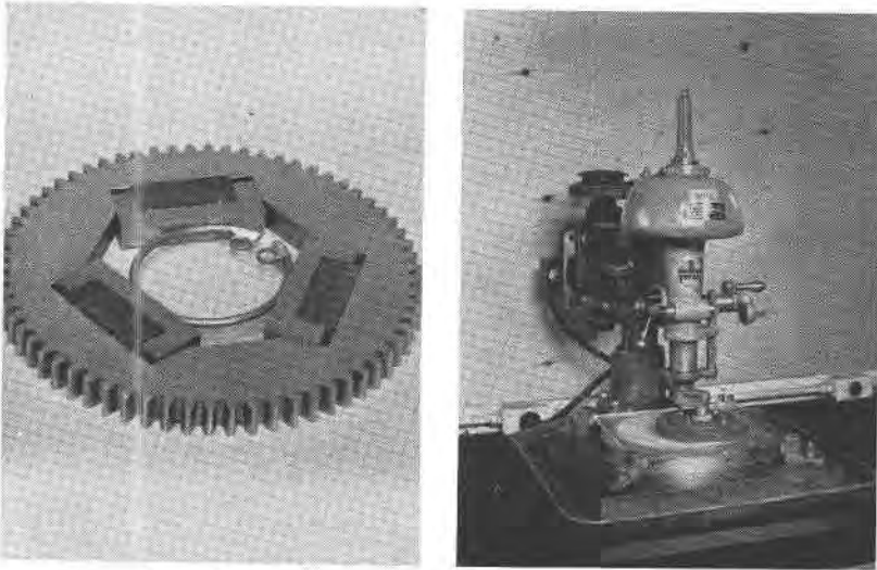
FIG. 15. Planetary lap gear for squaring crystals. Loaves of blanks are loaded in special gears and two surfaces lapped at once. Loaf is turned over for lapping other pair of sides. Method has extraordinary production capacity.
