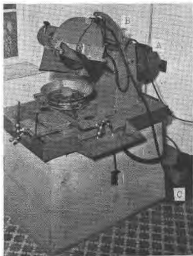
FIG. 2. Felker saw mounted on concrete block. (A) Adjustable counterweight; (B) depth stop; (C) coolant tank and circulating pump.
