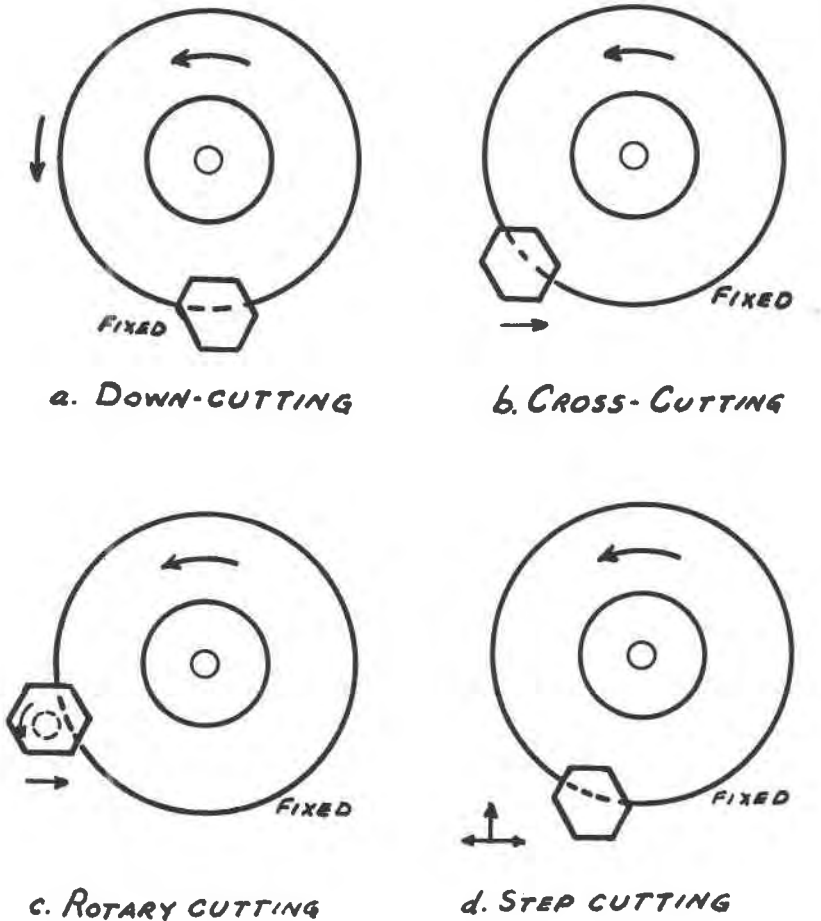
FIG. 1. Sawing methods. Down-cutting is the most widely used and successful method. The methods and equipment used in the diamond industry were found to be totally inadequate for quartz.
