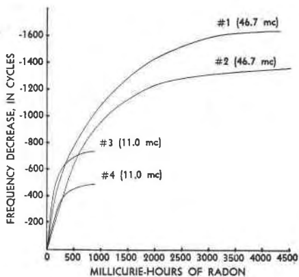
FIG. 10. Frequency change produced by radon in plated suspension mounted 8163 Kc plates. Container volume 57 cc.
