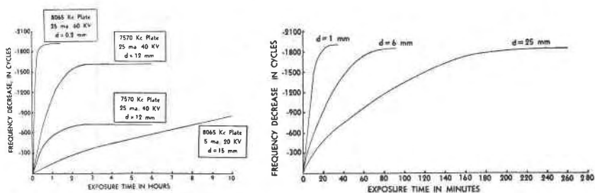
FIG. 4. Curves illustrating the variation in rate of change of frequency with x -ray beam intensity.
