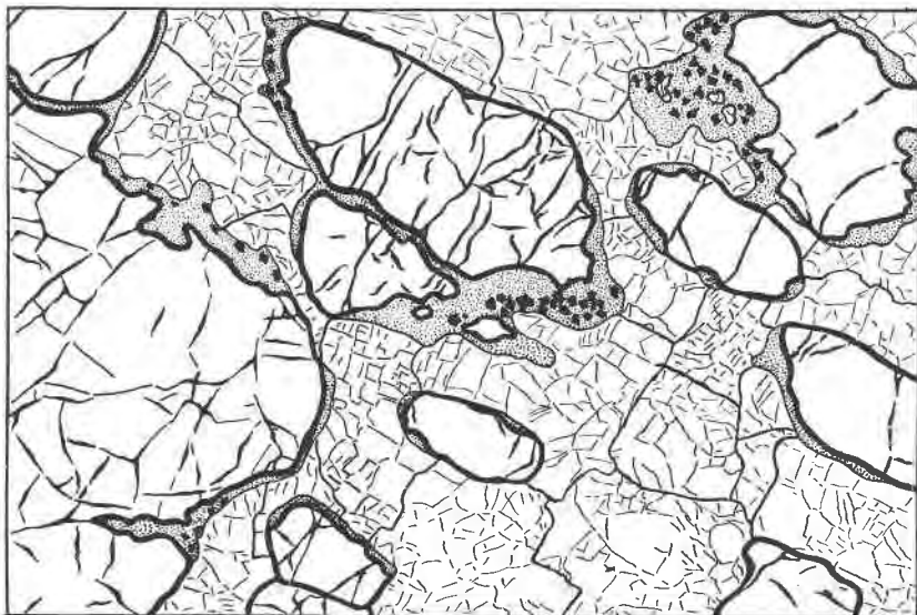
FIG. 1. Sketch of micro-section of eclogite ( \times 9 ) showing garnet with kelyphitic reaction zones. Opaque areas represent almandine spinel in the outer regions of the reaction borders. Omphacite forms the groundmass.
