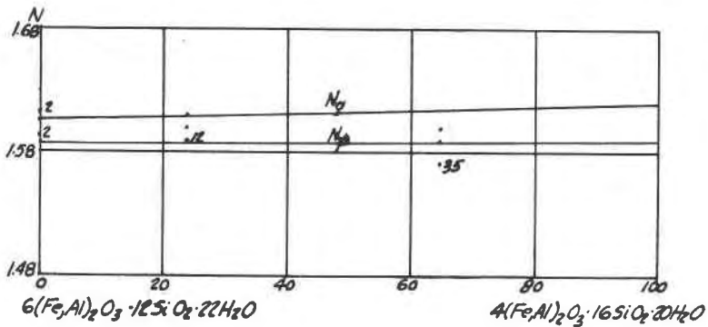
FIG. 4. Indices of refraction of montmorillonites (or nontronites) with much Fe 2 O 3 (between 10 and 13% atomic Al).
