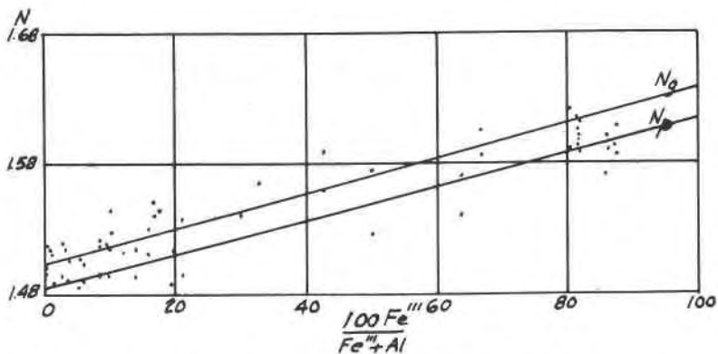
FIG. 6. Indices of refraction of montmorillonites with varying replacement of Al by Fe.
