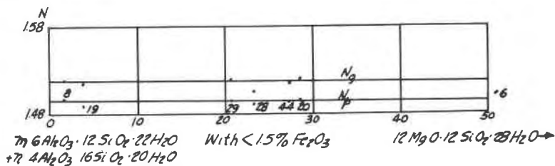
FIG. 5. Indices of refraction of montmorillonites (containing less than 1.5% \text{Fe}_2\text{O}_3 ) with varying replacement of Al by Mg.
