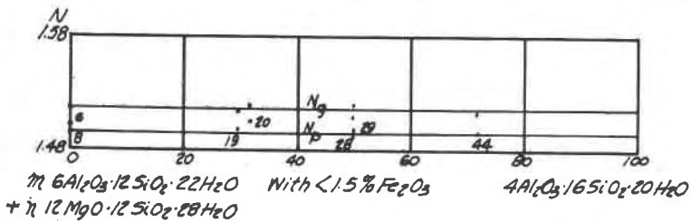
FIG. 3. Indices of refraction of montmorillonites (containing less than 1.5% Fe 2 O 3 ) with varying replacement of Si by Al.
