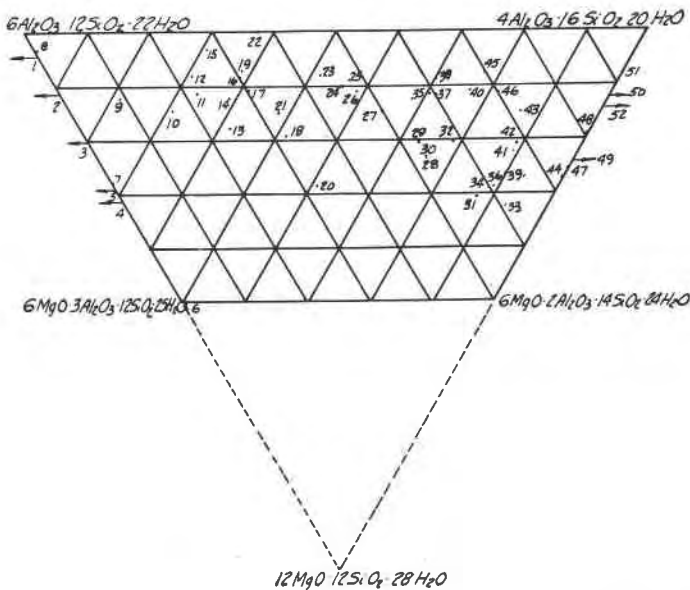
FIG. 1. Montmorillonite analyses plotted on (part of) a triangle having 4\text{Al}_2\text{O}_3 \cdot 16\text{SiO}_2 \cdot 20\text{H}_2\text{O} , 6\text{Al}_2\text{O}_3 \cdot 12\text{SiO}_2 \cdot 22\text{H}_2\text{O} , and 12\text{MgO} \cdot 12\text{SiO}_2 \cdot 28\text{H}_2\text{O} at its corners, Al standing for Al, Fe III , Ti and Cr, and Mg for Mg, Fe II , Mn, Ca.
