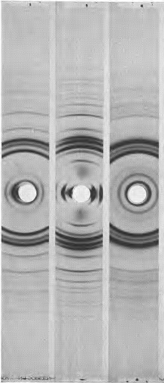
FIG. 5. X-ray powder photographs of the soap crystal types discussed in this paper. These photographs were taken with a camera having the standard diameter of 114.6 mm. (on which 1 mm. film distance corresponds to 1^\circ for the deviation angle, 2\theta , and to \frac{1}{2}^\circ for the Bragg angle, \theta ). For purposes of comparison by others, these photographs are reproduced here to exactly natural size. (The middle photograph displays severe orientation which cannot be eliminated by fine-grinding the sample, since grinding causes the transformation \alpha \rightarrow \beta to occur.)
