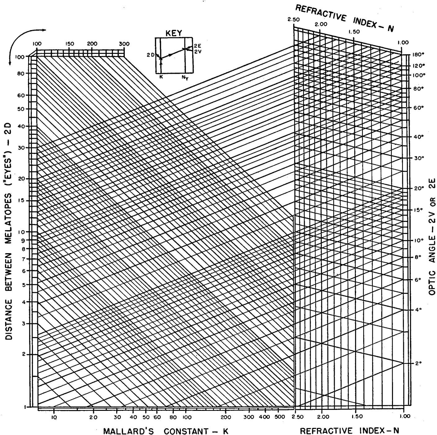
FIG. 1. Chart of 2D/2 = K \sin(2E/2) = N\gamma K \sin(2V/2) .
