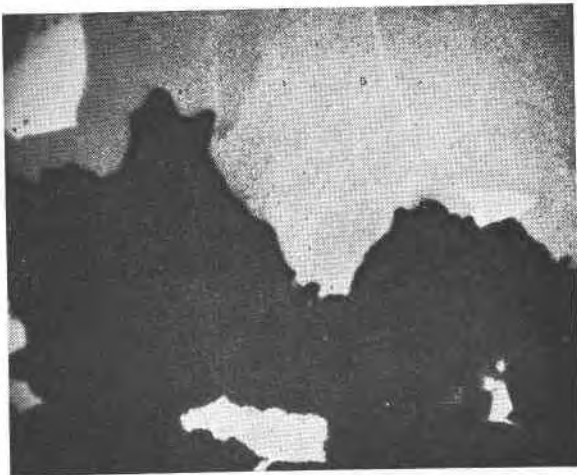
FIG. 3. Deposition of Radiocolloids Along Interface. Detail from alpha ray pattern (10X) showing zone of radiocolloid deposition (black) between uraninite (dark gray) and uranophane (light gray). The white inclusions are cyrtolite whose feeble radioactivity is not reproduced in the print. The zone of high alpha ray activity is revealed as a fine line of lead dithizonate on the ammonium acetate-lead pattern. Specimen collected by author at Spruce Pine, Mitchell Co., N.C.
