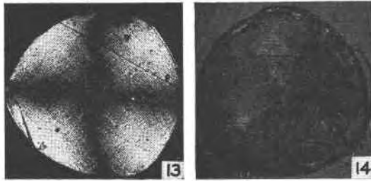
FIG. 13. Cross section of rod-shaped artificial spinel boule, as received. Polarized light. Crossed polaroids. Mag. 11×.
