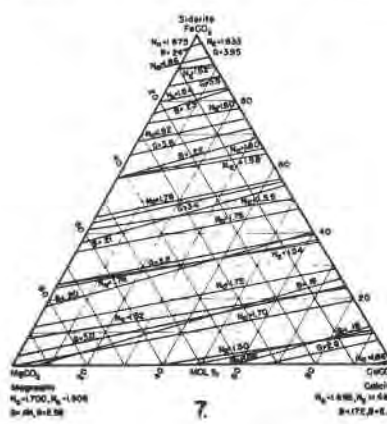
FIGS. 5, 6. Properties of CaCO_3-ZnCO_3-FeCO_3 without (5) and with (6) B/D lines. FIGS. 7, 8. Properties of FeCO_3-MgCO_3-CaCO_3 without (7) and with (8) B/D lines.
