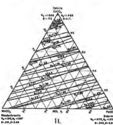
FIGS. 9, 10. Properties of \text{CaCO}_3\text{-MnCO}_3\text{-ZnCO}_3 without (9) and with (10) B/D lines. FIGS. 11, 12. Properties of \text{CaCO}_3\text{-MnCO}_3\text{-FeCO}_3 without (11) and with (12) B/D lines.
