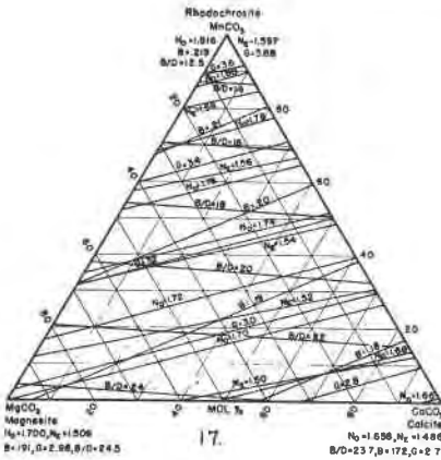
FIG. 17. Properties of MnCO 3 -MgCO 3 -CaCO 3 . FIG. 18. Properties of ZnCO 3 -CaCO 3 -MgCO 3 .
