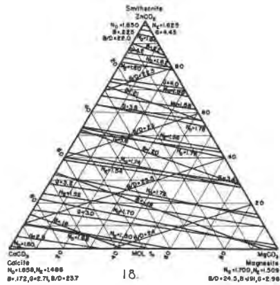
FIG. 17. Properties of MnCO 3 -MgCO 3 -CaCO 3 . FIG. 18. Properties of ZnCO 3 -CaCO 3 -MgCO 3 .
