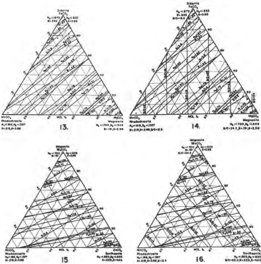
FIGS. 13, 14. Properties of FeCO 3 -MnCO 3 -MgCO 3 without (13) and with (14) B/D lines.
