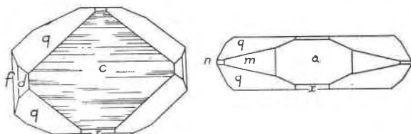
FIG. 1. Two views of a crystal of paraschoepite.
