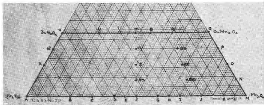
FIG. 1. Synthetic preparations within the system.
