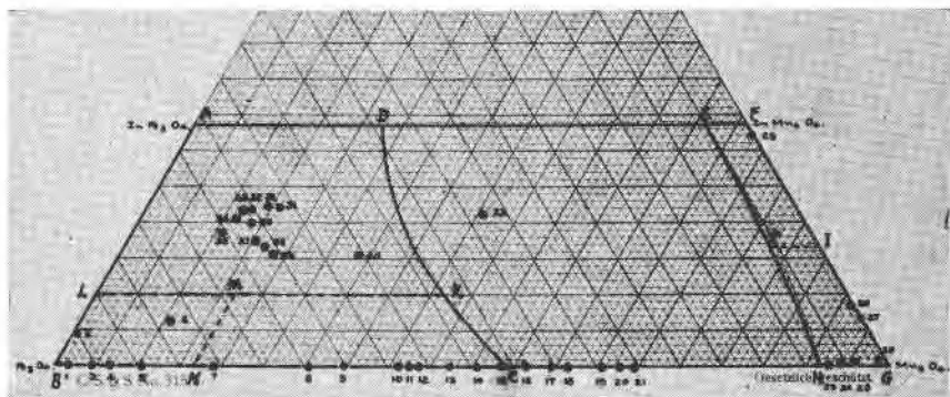
FIG. 7. Analyses of minerals falling within the system, and suggested composition limits for the different species. Magnetite BNML ; jacobsite NMKC ; franklinite ADKL ; vredenborgite DEHC ; hetaerolite EFIJ ; hausmannite GHII .
