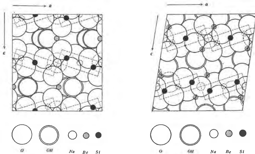
FIG. 6. The structure of epididymite (left) contrasted to that of eudidymite (right). The positions of atoms are displaced from their true positions to ideal positions to reveal the relationship of the two structures. Projections on (010).
