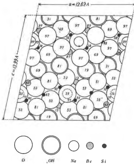
FIG. 5. The structure of eudidymite, projected on (010). Numbers given in decimal fractions of the b -length are the height of atoms.
