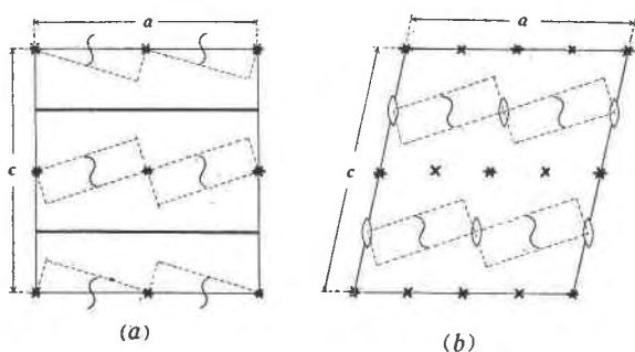
FIG. 4. The \text{Si}_3\text{O}_8 groups arranged in the space group V_h^{16} (epididymite) and in the space group C_{2h}^6 (eudidymite). Dotted rectangles represent the \text{Si}_3\text{O}_8 groups. Crosses and asterisks represent centers of symmetry. Heavy full lines represent the traces of reflection planes. Other symbols as in common use. Projections on (010). (a) epididymite; (b) eudidymite.
