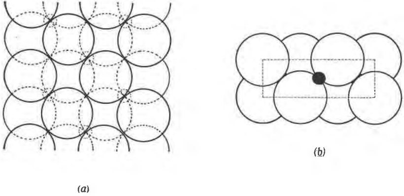
FIG. 2. \text{Si}_3\text{O}_8 -chain. Large circles represent oxygen atoms and small circles silicon atoms (a) plan; (b) elevation (as viewed from the chain-direction).
