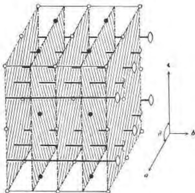
FIG. 1. Symmetry elements of the space group C_{2h}^6-C2/c . Small white and black circles represent centers of symmetry. Shaded planes represent glide planes.
