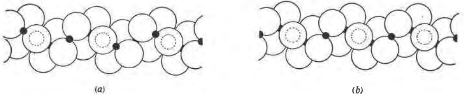
FIG. 3. Two different modes of forming a \text{NaSi}_3\text{O}_7 sheet. Large circles represent oxygen atoms, medium sized circles represent sodium atoms, and small circles represent silicon atoms. (a) epididymite; (b) eudidymite.
