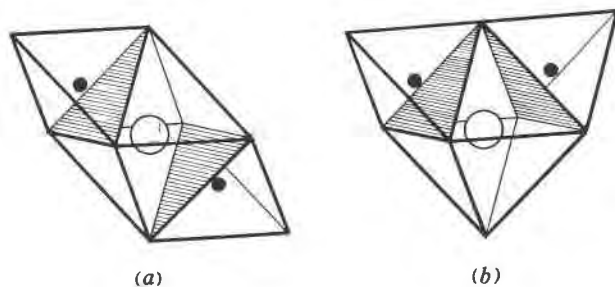
FIG. 7. Tetrahedral groups adjoining an octahedral group of oxygen atoms in epididymite (a) and in eudidymite (b). Common faces are shaded. Large open circles represent sodium atoms. Small black circles represent silicon atoms. Oxygen atoms, lying on the octahedral and tetrahedral corners are omitted.
