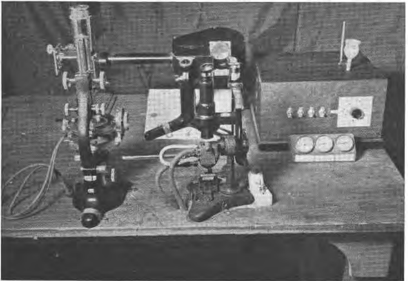
FIG. 3. Relation of heating unit to microscope and refractometer.
