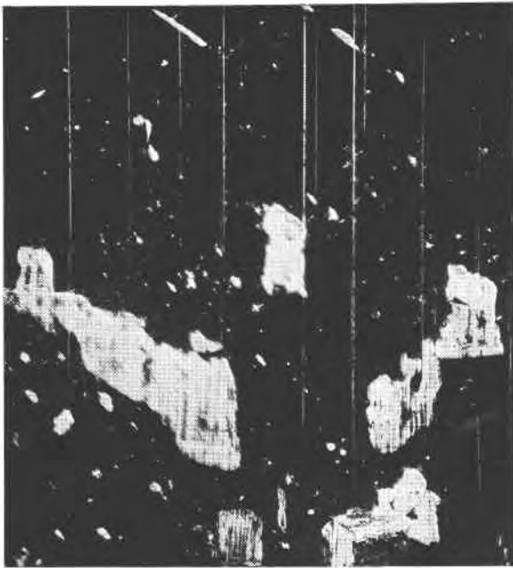
FIG. 5. ( \times 60 ) Photomicrograph of a thin section of the feldspar cut parallel to (001) to show newly formed albite ( Ab_{95}An_5 ) with relict microcline.
