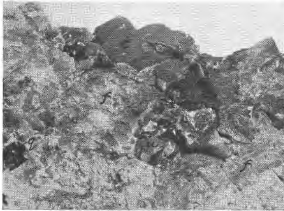
FIG. 1. ( \times 2 ) Uraninite ( u ) crystal on matrix of feldspar ( f ) (albite, Ab_{95}An_5 ), with columbite ( c ), and quartz ( q ).
