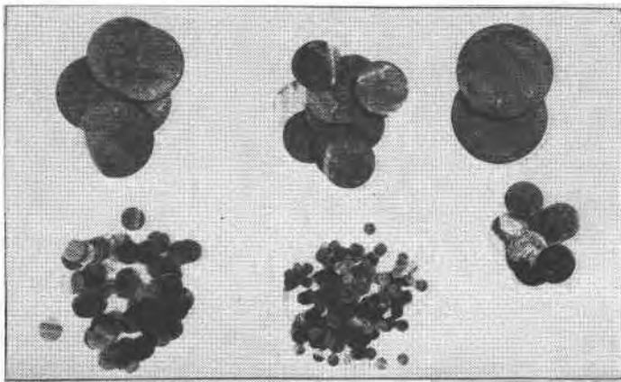
FIG. 8. Selection of lapped tourmaline discs, ranging in thickness from 0.015 inch in the smallest size ( \frac{1}{4} inch diameter) to about 0.070 inch in the largest ( 1\frac{7}{8} inch diameter).
