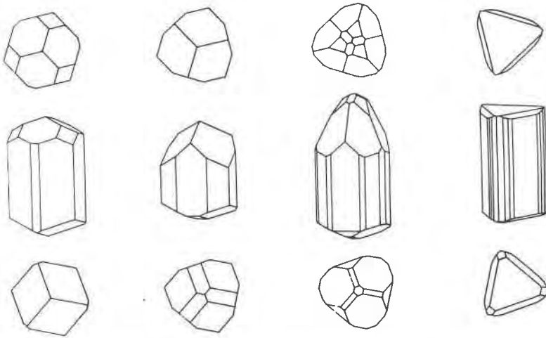
FIG. 2. Some typical habits of tourmaline crystals. Basal projections are given of the antilogous (above) and analogous (below) poles.
