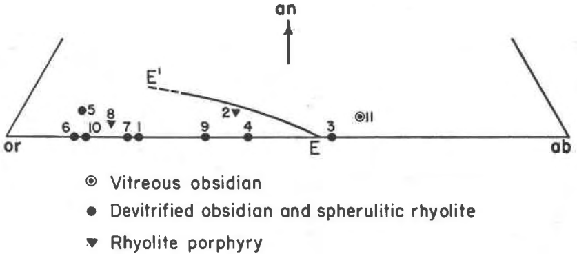
FIG. 1. Normative feldspar content of rhyolitic rocks of the Esterel.
