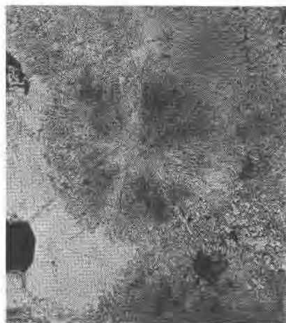
FIG. 3.—Spherulitic Rhyolite.
