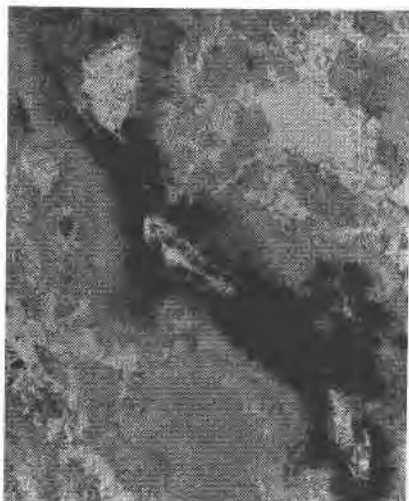
FIG. 2.—Spherulitic Rhyolite.
