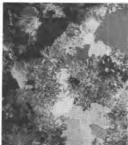
FIG. 4. Spherulitic Rhyolite.
