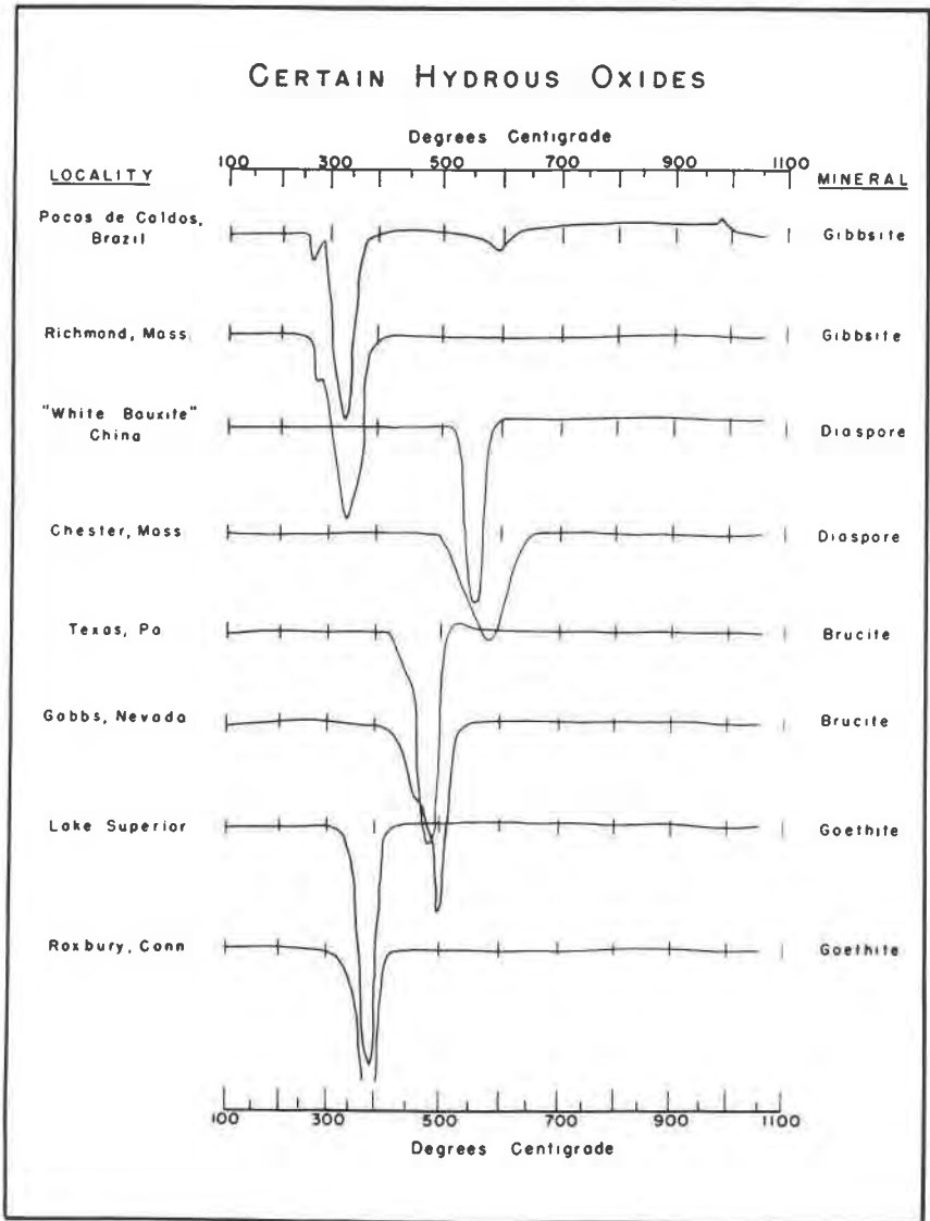
FIG. 9. Curves of gibbsite, diaspore, brucite and goethite are shown for comparison.
