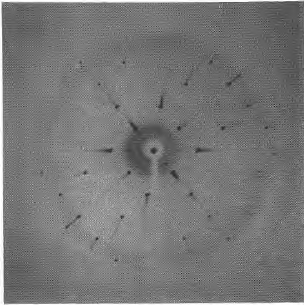
FIG. 9. Lindgrenite, b axis, zero level (Mo) (new c^* horizontal)
