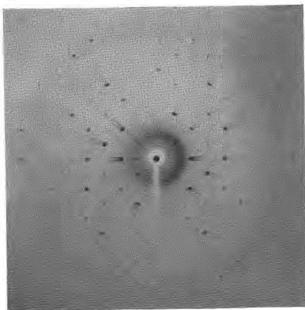
FIG. 4. Lindgrenite, b axis, first level (Mo) ( c^* horizontal)
