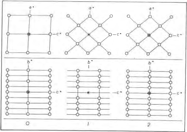
FIG. 5. 0,1,2 level reciprocal lattice nets shown by (upper row) b and (lower row) a axis precession photographs of lindgrenite. (Diffraction symbol (2/M)B(2_1/c) .)
