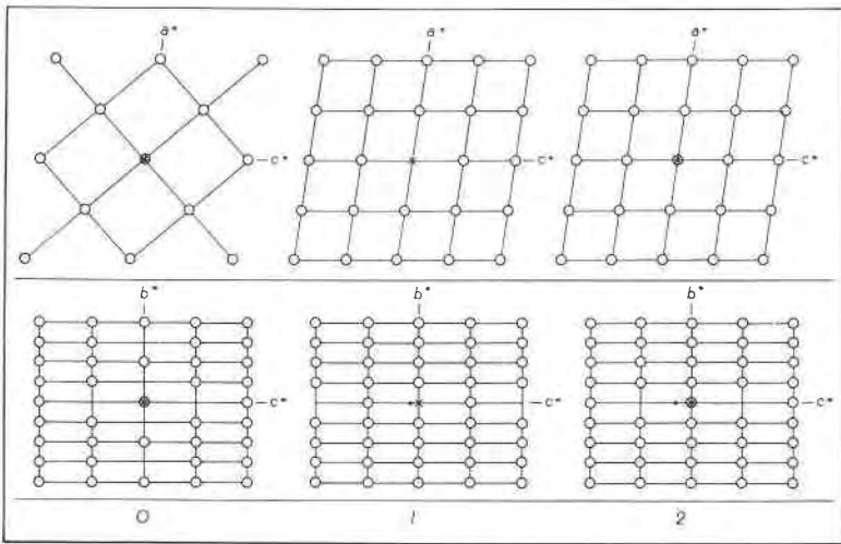
FIG. 11. 0, 1, 2 levels reciprocal lattice nets shown by (upper row) b and (lower row) a axis precession photographs of lindgrenite.
