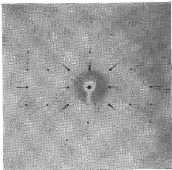
FIG. 3. Lindgrenite, b axis, zero level (Mo) ( c^* horizontal)
