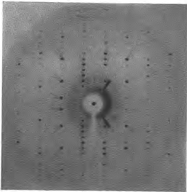
FIG. 2. Lindgrenite, a axis, first level (Mo) ( c^* horizontal)
