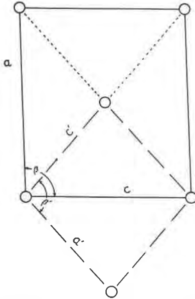
FIG. 6. Lindgrenite. Base of b -end centered cell ( a, c, \beta ), full lines, and base of primitive cell ( a', c', \beta' ), broken lines.
