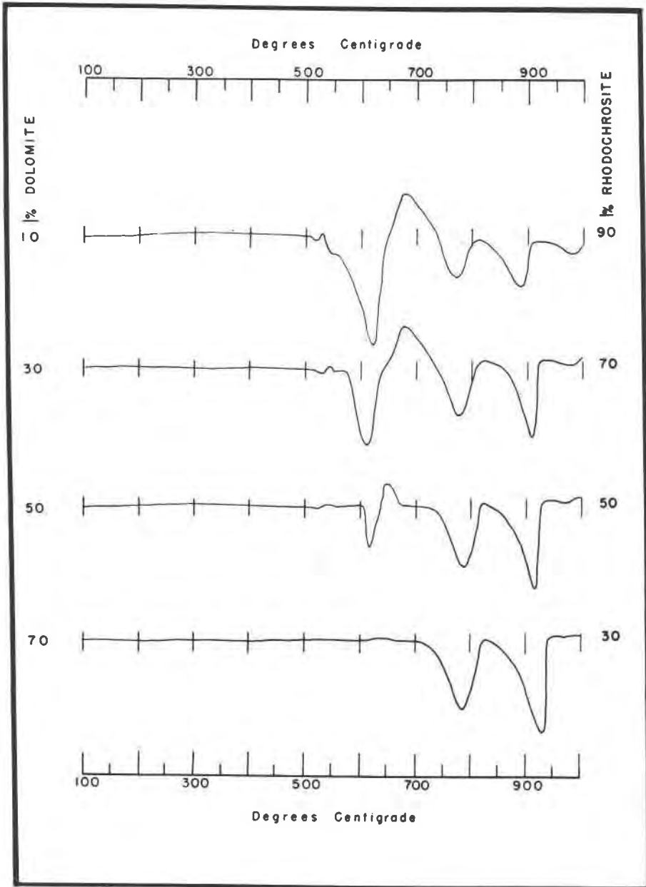
FIG. 4. Differential Thermal Curves of Mixtures of Rhodochrosite with Dolomite.
