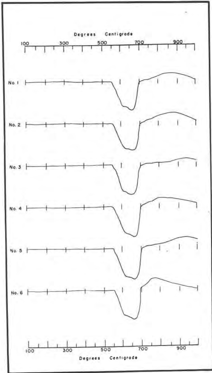
FIG. 1. Exothermic Peak Study. Cover on, restricting free access of air to sample. (50-120 mesh fragments.)
