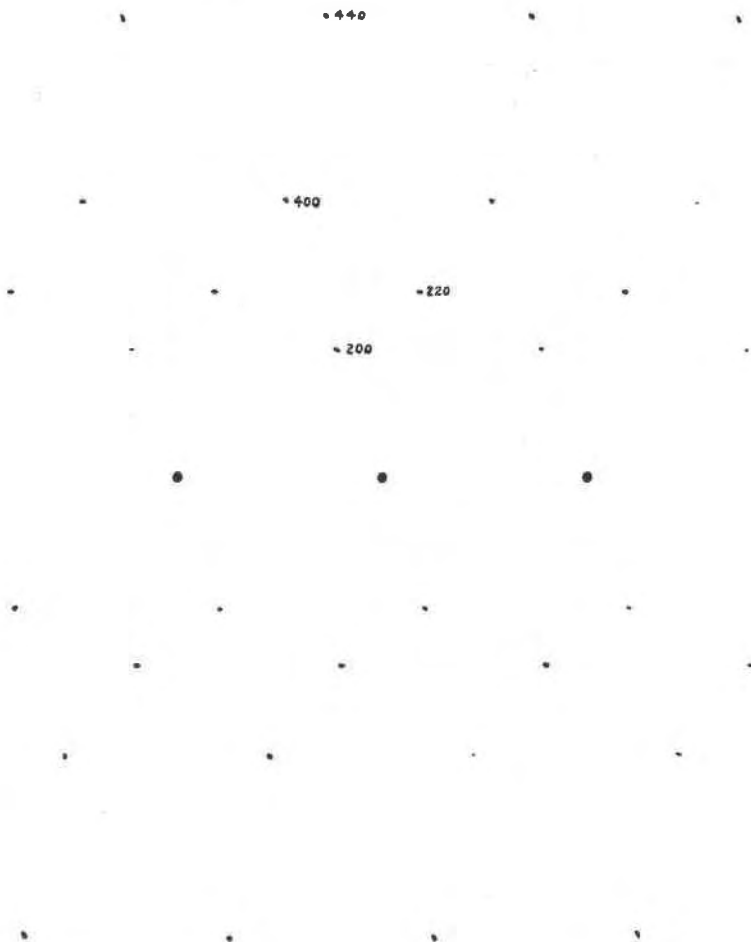
FIG. 1. Weissenberg photograph of the zero layer-line of a single crystal of bornite made with cobalt K\alpha -radiation. The direct beam spots along the center-line of the photograph indicate the translations of the film corresponding to 90^\circ of rotation of the crystal. The small light areas in the centers of the direct beam spots mark the outline of the crystal. The indices of the spots refer to the cubic cell of edge-length 5.47 \text{ \AA} .
