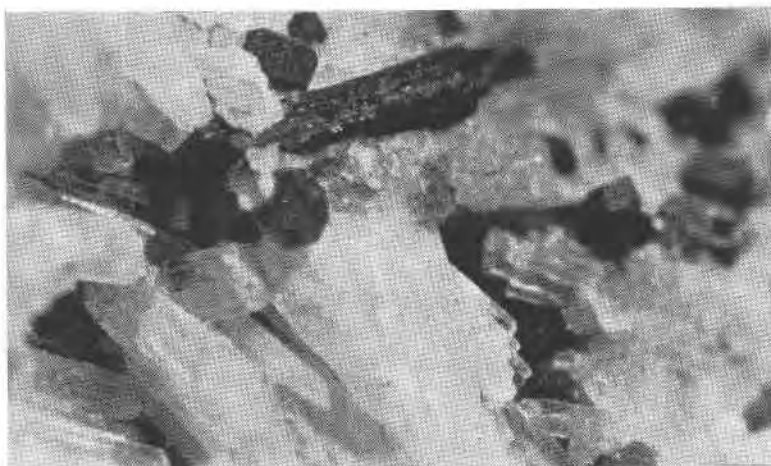
FIG. 2. x25. Glassy crystallized drusy natrolite, with rhombohedral andradite and prismatic allanite (upper center).
