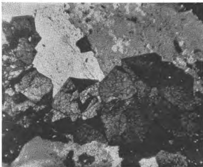
FIG. 4. This section \times 100 , crossed nicols. Andradite garnet and natrolite. Shows birefracting segments in andradite.
