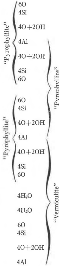
FIG. 4. Schematic representation of the sequence of atomic layers in rectorite.
